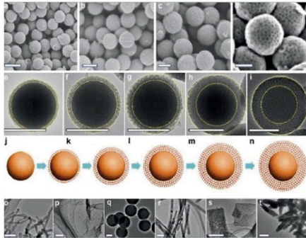
STEP 1. Process of transforming natural clay into PHOMI STONE
